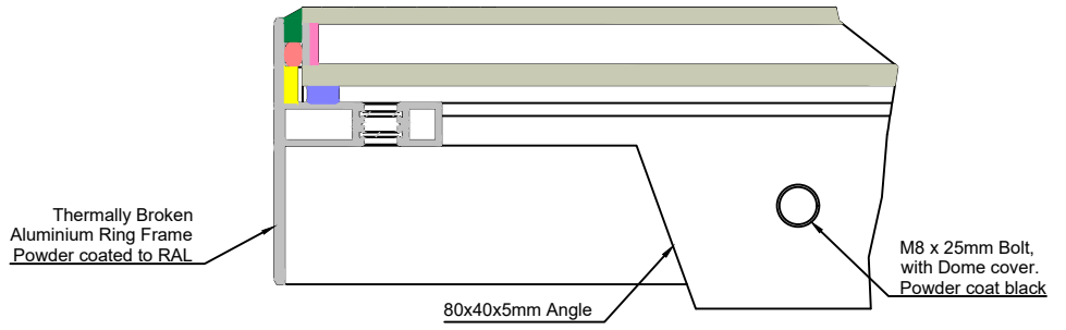
Detail E
